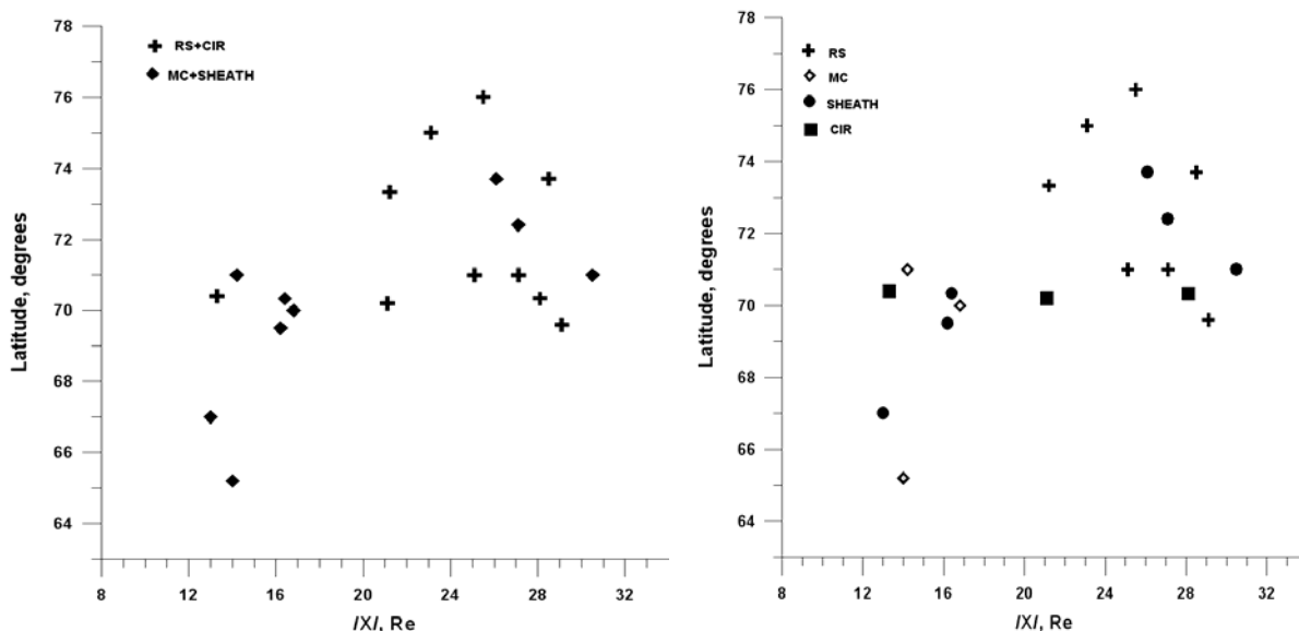
Figure 2. Latitude of the poleward edge of the aurora (seen by Polar UVI at the meridian of Geotail) as a function of the distance between Geotail and Earth at the moment of the flow reversal registration
