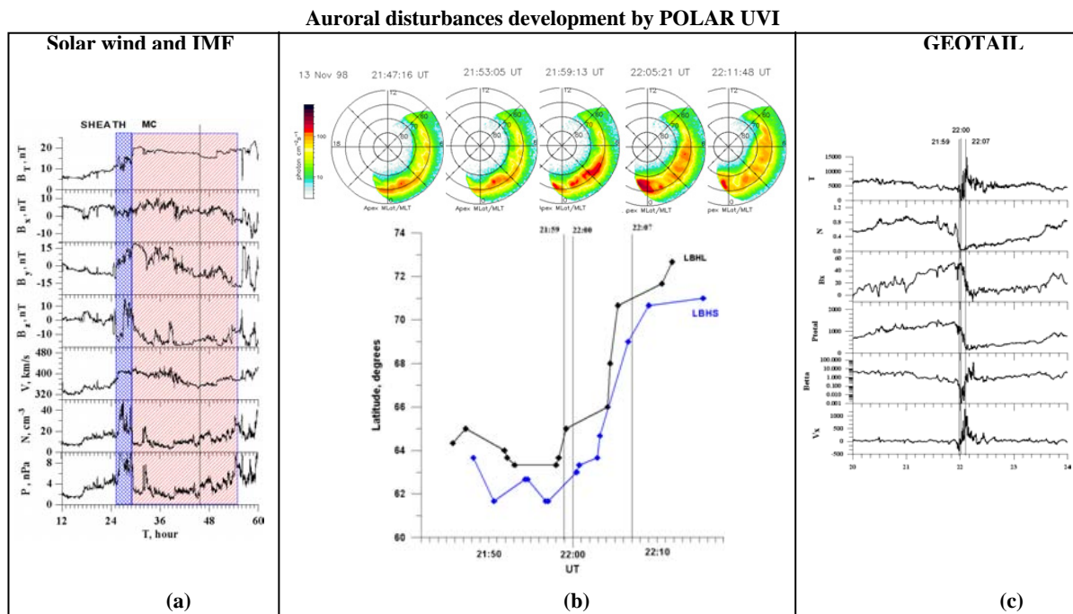
Figure 1. Auroral disturbances during the MC event on 13 November 1998.
